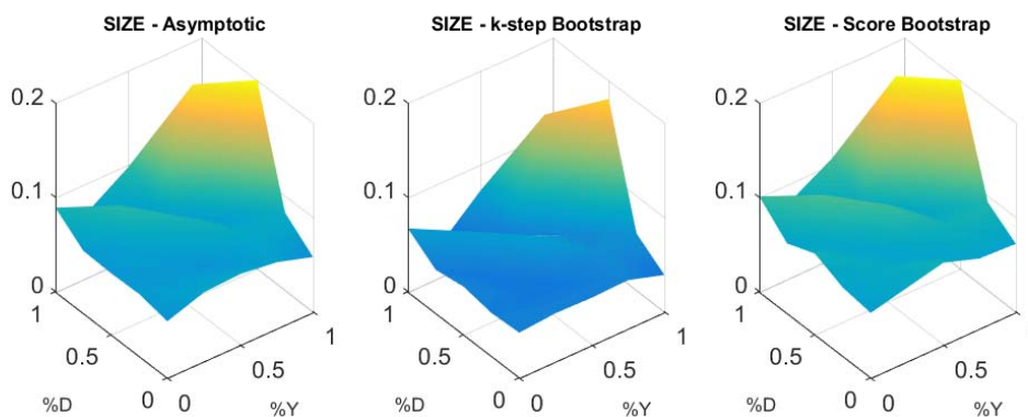
FIGURE 3. This figure shows the simulation size of 5% level tests based on the factor-lasso estimator in the IV partial factor model and the asymptotic Gaussian approximation, the k -step bootstrap, and a score based bootstrap. Size is shown in the vertical axis. The horizontal axes give the fraction of the explanatory power in an infeasible regression of Y on factors and factor residuals, “%Y,” and the fraction of the explanatory power in an infeasible regression of D on factors and factor residuals, “%D,” where the infeasible regressions are described in the text.
