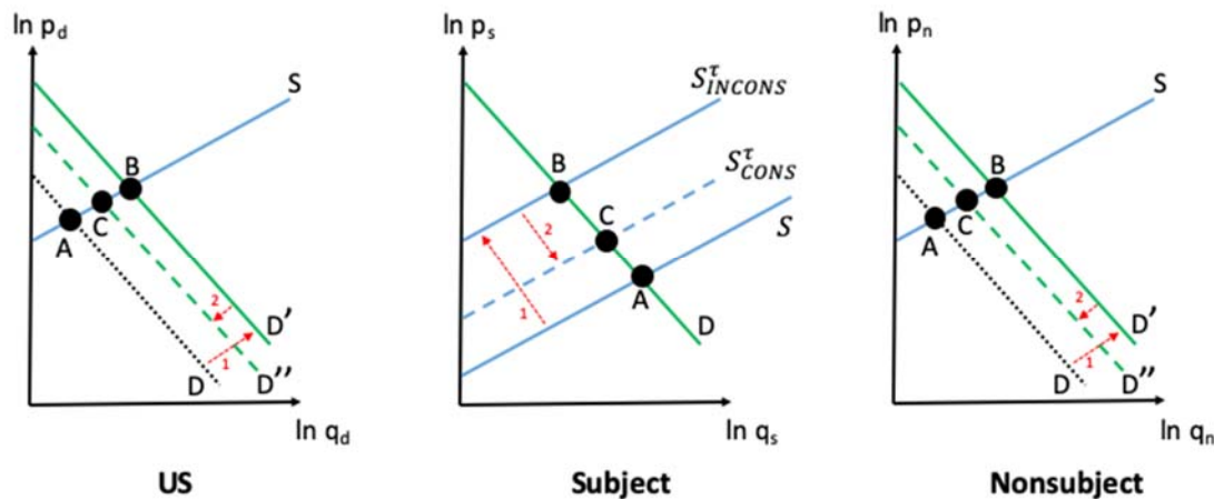
Figure 1 – Policy Analysis in an Armington Elasticities Model
