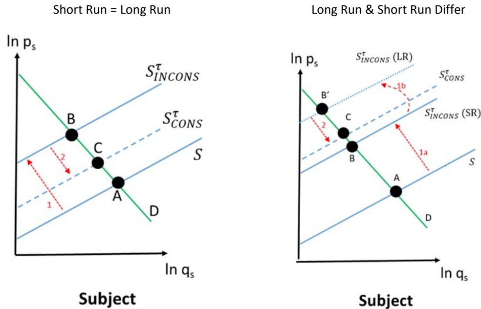
Figure 2 – Does Armington Model Capture Actual Market Dynamics?
